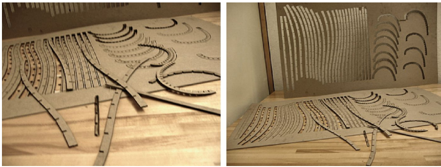
Figure 1. Laser-cut sheets of cardboard
