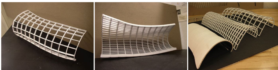
Figure 1. Assembled prototypes with various rib densities.
