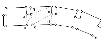
Figure 4. Flattening pattern based on triangular strips.
